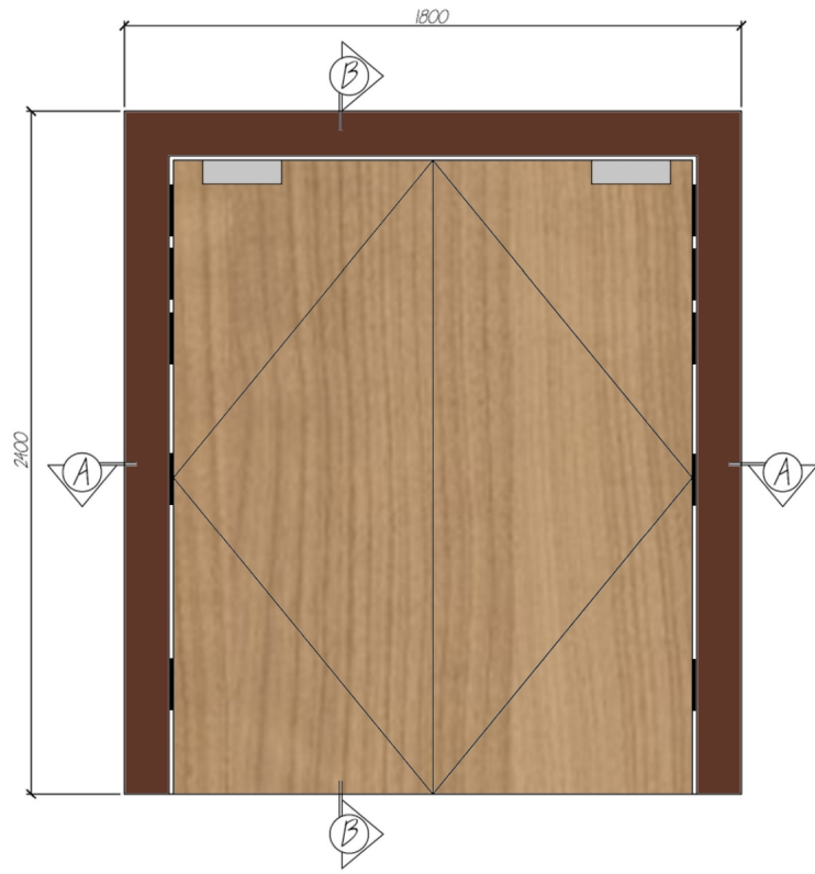
AWP DOUBLE LEAF TIMBER ACODOR
